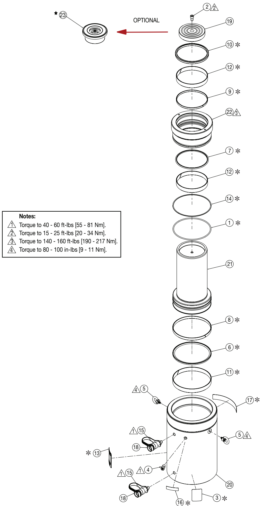
Figure 2, Exploded View - Model HCR-250 Tall
