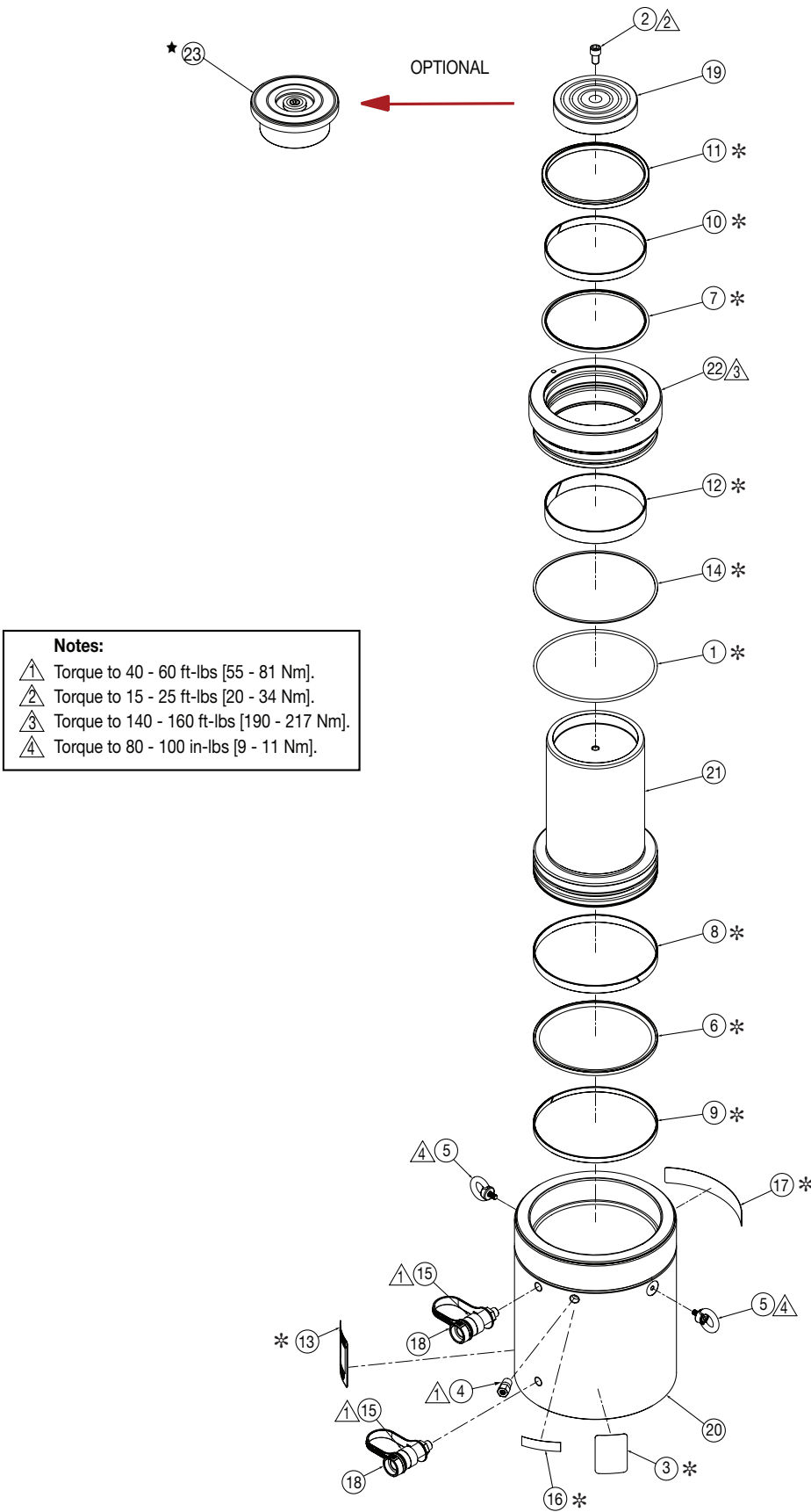
Figure 1, Exploded View - Model HCR-250 Short
