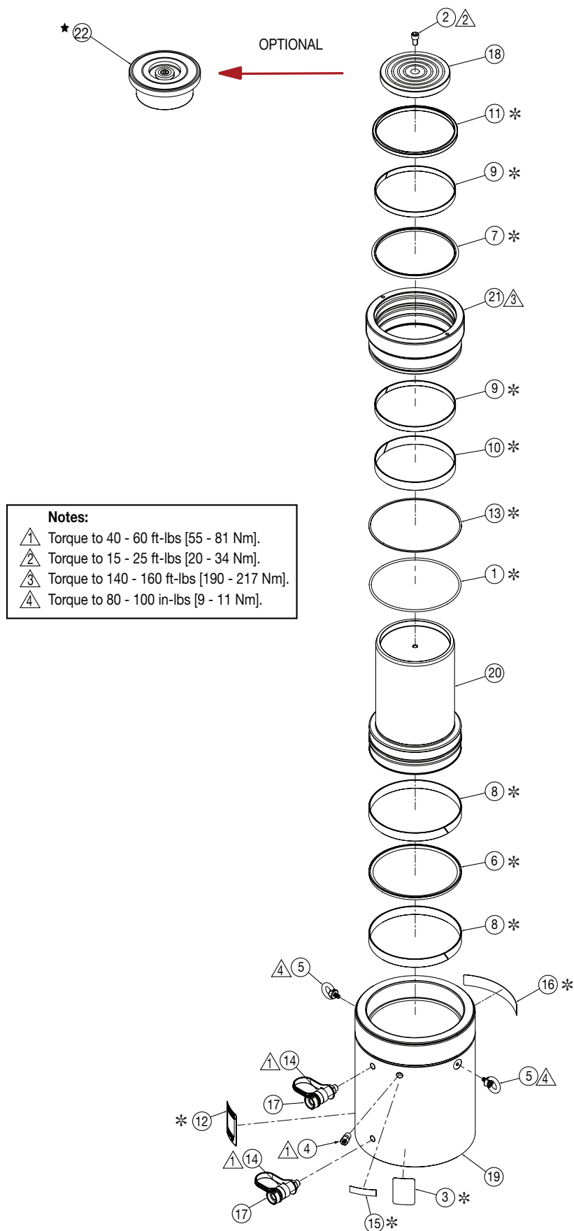
Figure 3, Exploded View - Model HCR-300
