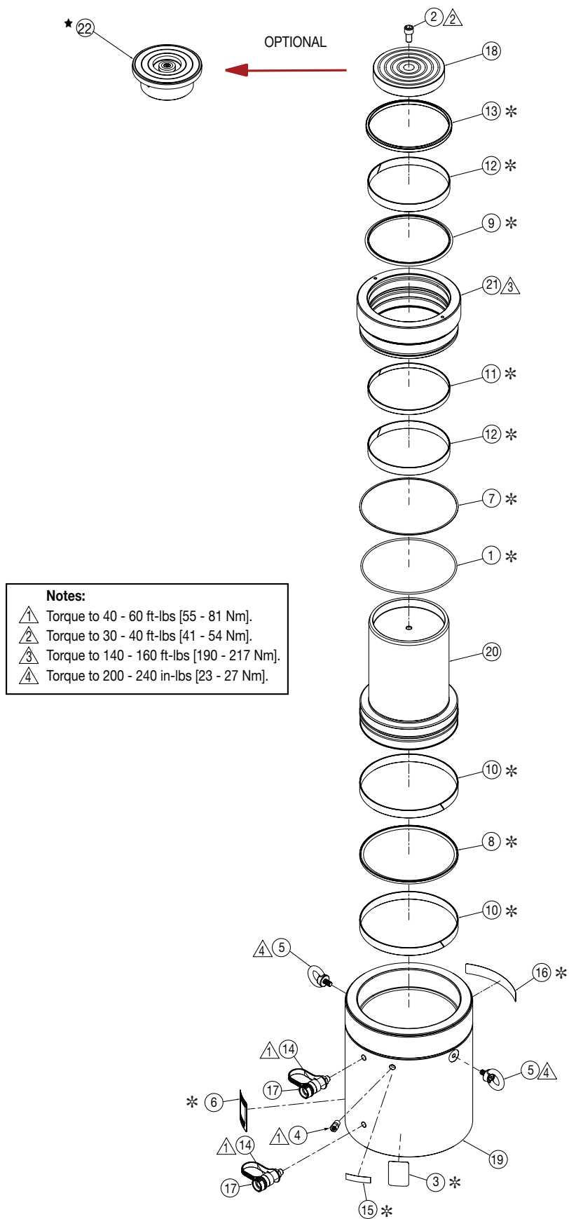
Figure 4, Exploded View - Model HCR-400
